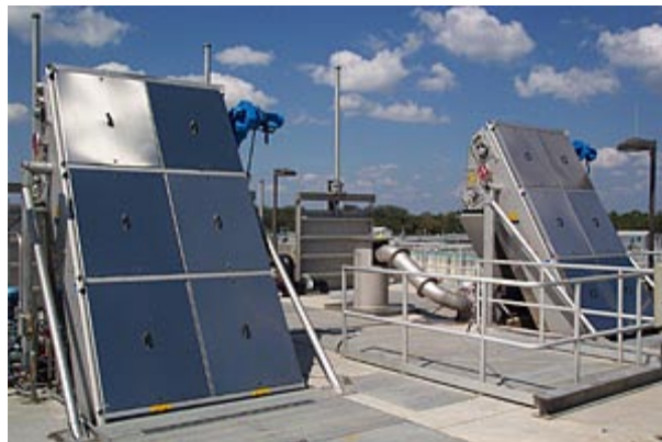
Huber Technology EscMax ® perforated plate screen
